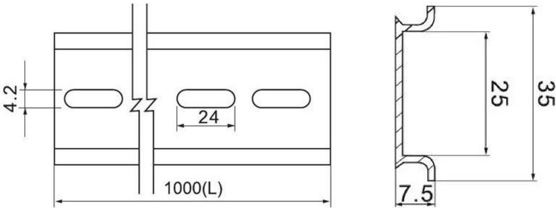
GK6800A/B LMITATION IMPORTED LONG HOLE
